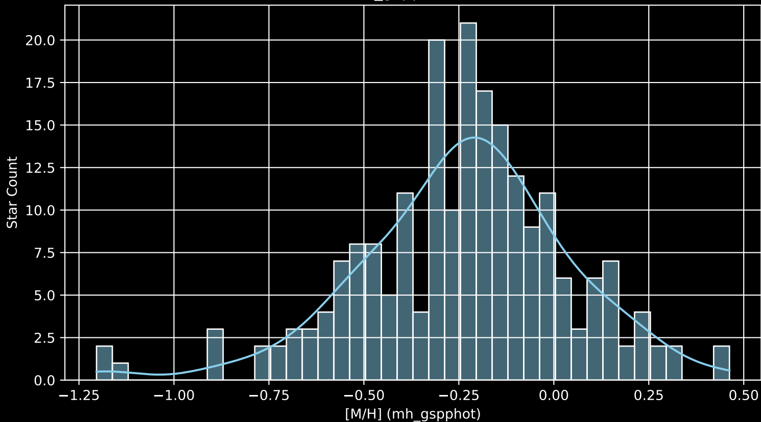
APOGEE DR17 Field: [059-41_MGA [M/H] (mh_gspphot) (n= 212)
