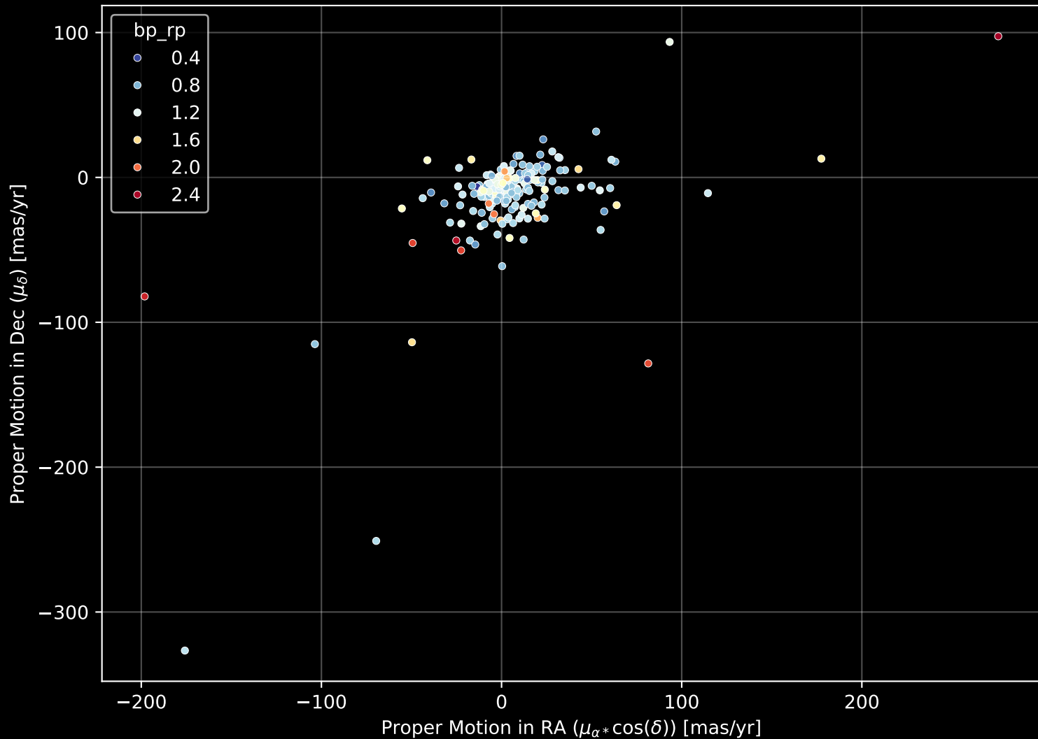
APOGEE DR17 Field: [059-41_MGA] Proper Motion Diagram (n= 212)
