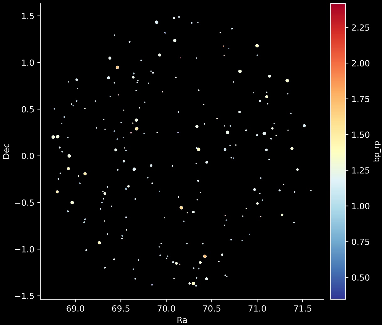
APOGEE DR17 Field: [059-41_MGA] Stars: 212
