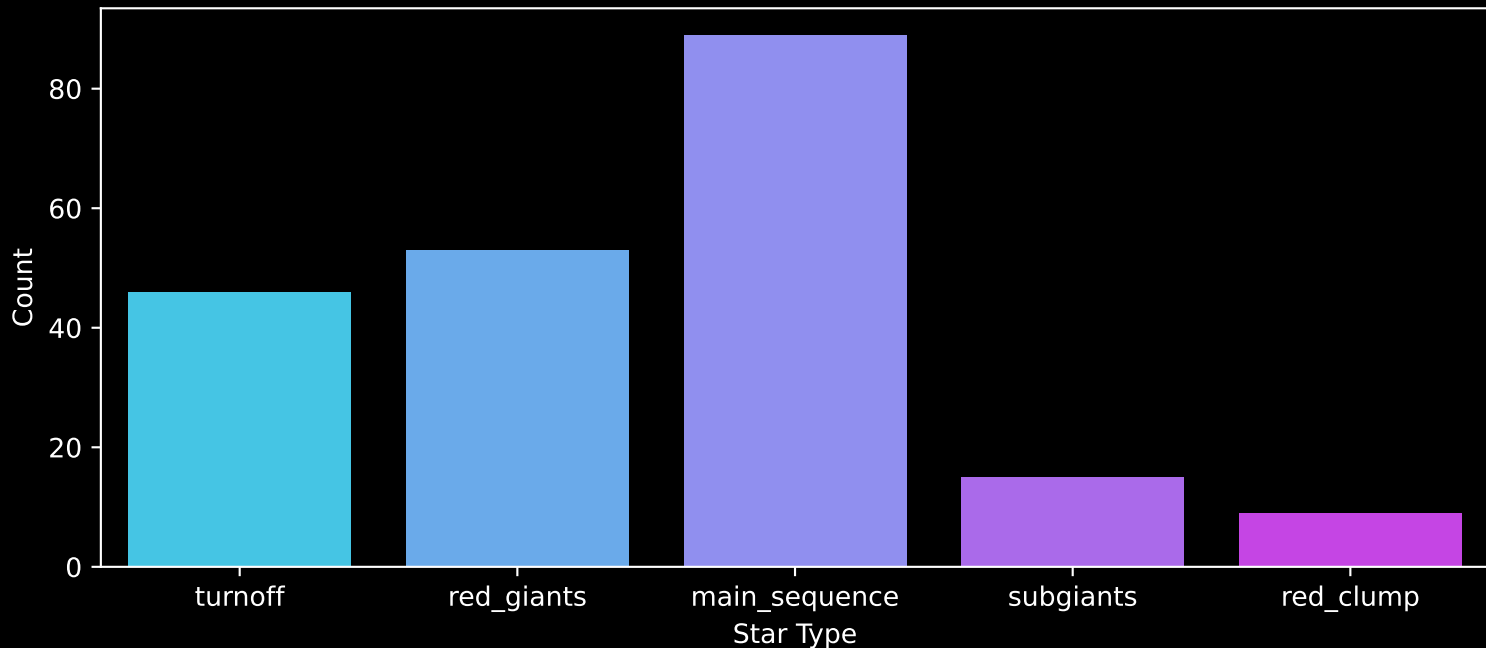
APOGEE DR17 Field: [059-41_MGA] Count plot of Star Type
