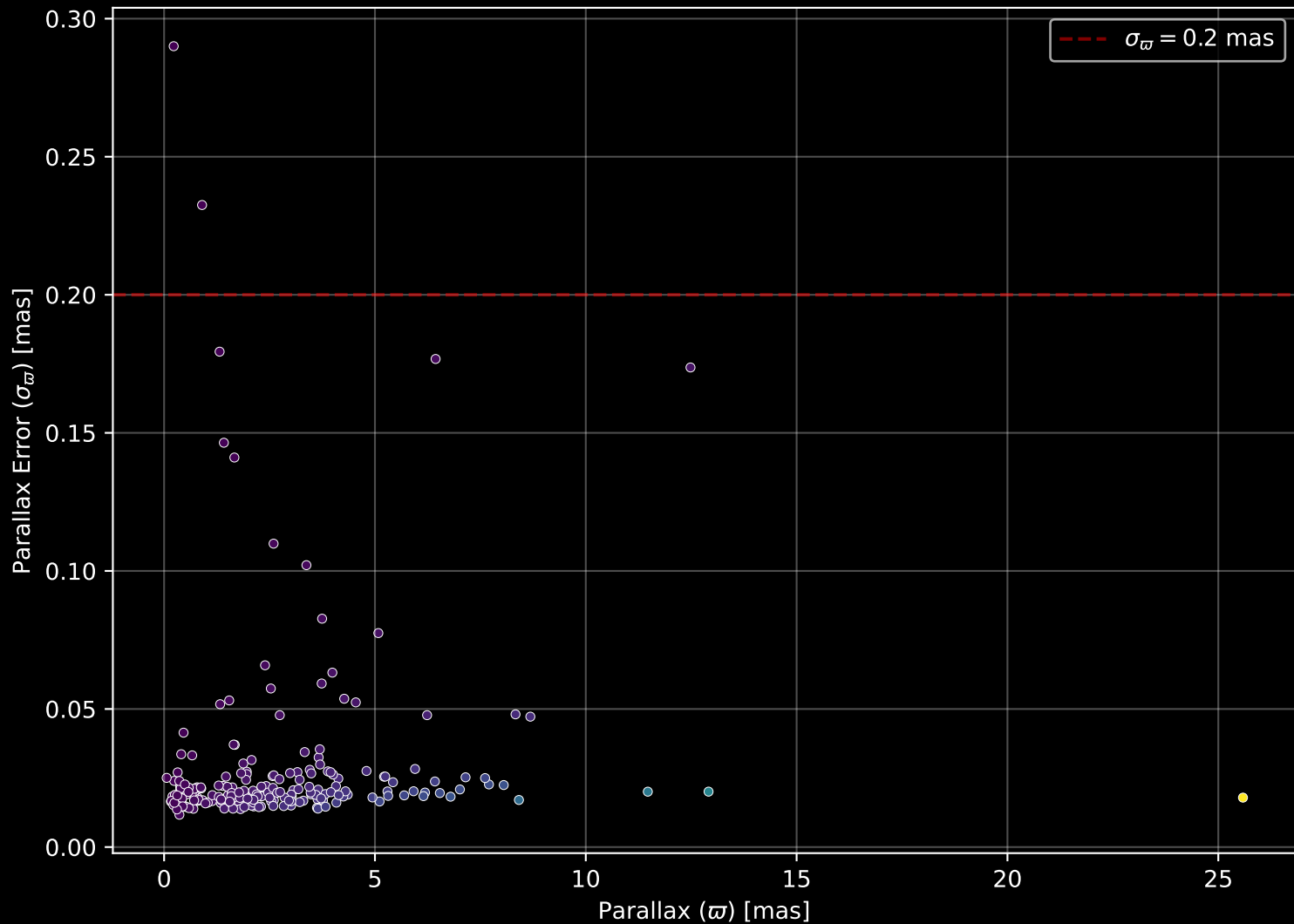
APOGEE DR17 Field: [059-41_MGA] Parallax Quality (n= 212)
