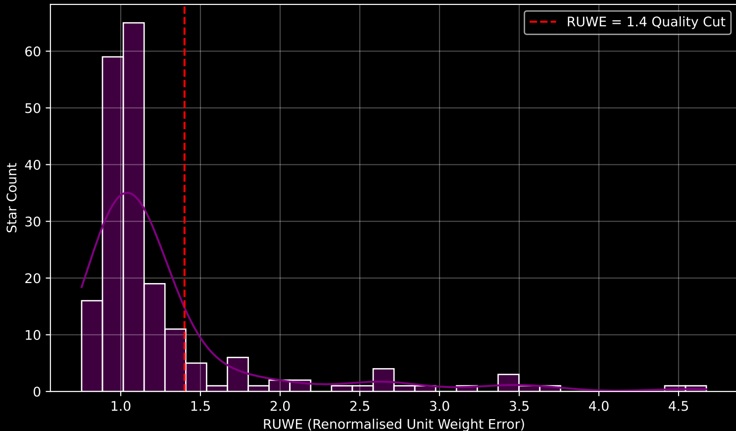
GAPOGEE DR17 Field [059-41_MGA] RUWE Distribution (n= 203)
