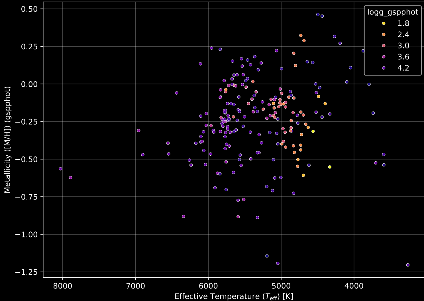
APOGEE DR17 Field: [059-41_MGA] Stellar Population Parameters (n= 212)
